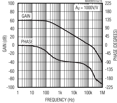
GAIN AND PHASE vs. FREQUENCY ( R_L = 5k\Omega , C_{LOAD} = 100pF )
